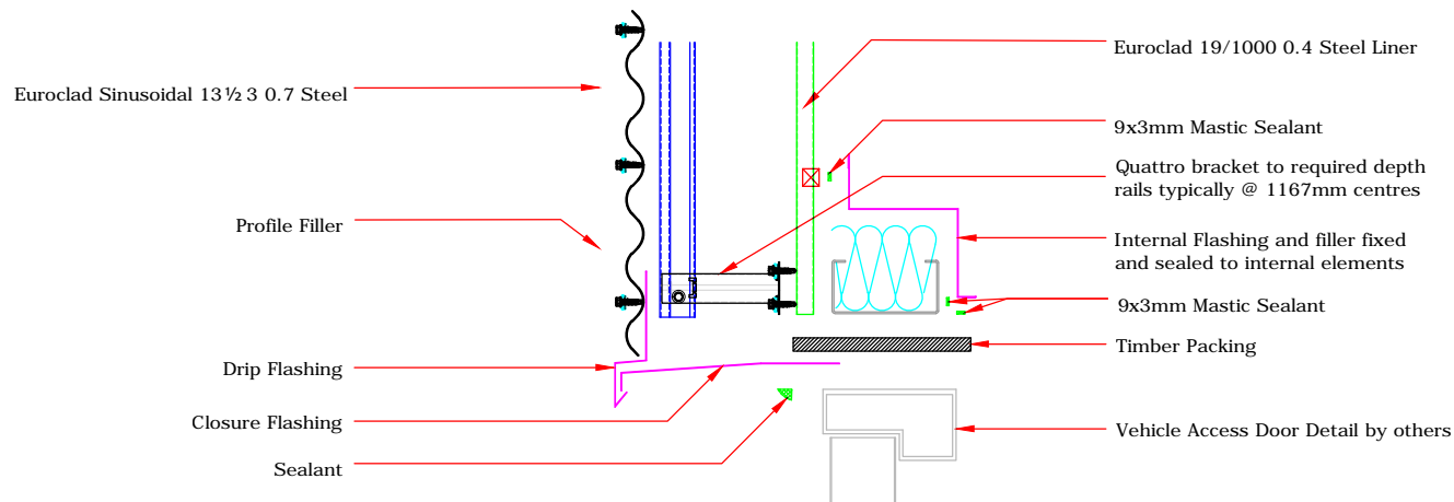
EUROCLAD ELITE SYSTEM 57 WALL CONSTRUCTION
